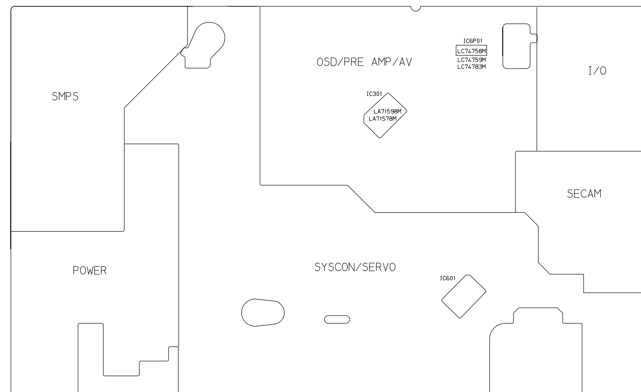
Conductor Side
