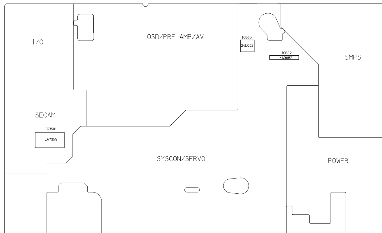
Component Side
